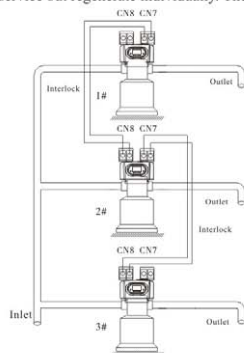
Figure 3-12 Interlock system
