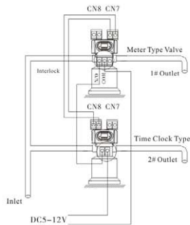
Figure 3-13 Series system
