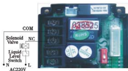
Figure 3-2 Wring of Solenoid Valve on Outlet
