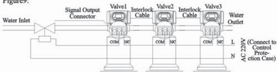
Figure 9 Wiring of Solenoid Valve in Inlet
